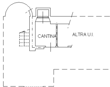
PIANO INTERRATO H=ml. 2.55
